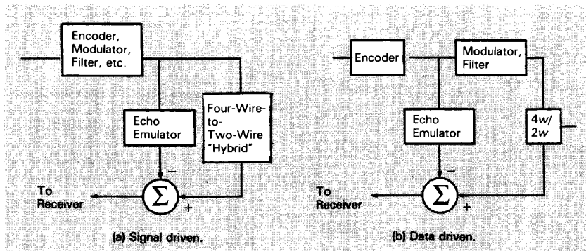
Fig. 8. Echo cancelers.
